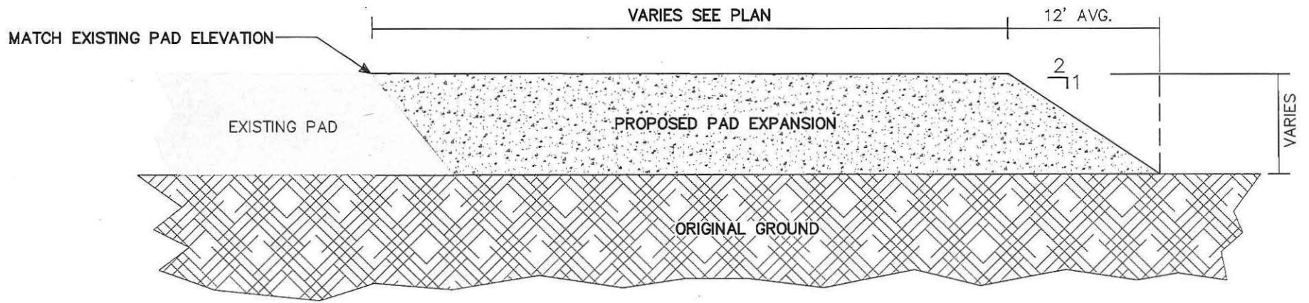
(TYPICAL PAD EXPANSION CROSS-SECTION A-A DETAIL) SCALE: N.T.S.
